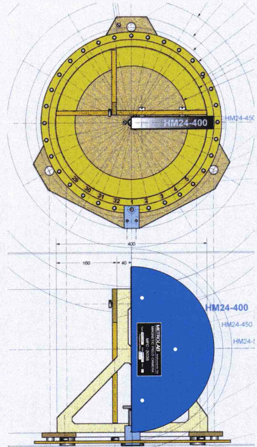
Vertical mounting MFC 3040
