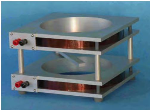
Figure 2 (left and below): An example of a modern-day industrial fluxmeter, with a Helmholtz coil to measure the magnetic dipole of permanent magnets. Images courtesy of Magnet-Physik Dr SteinGroever, Cologne, Germany
